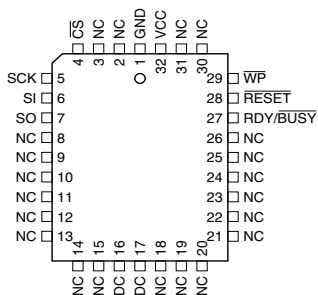
PLCC
